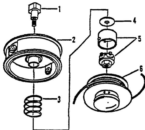
21560050 ECHOMATIC HEAD
