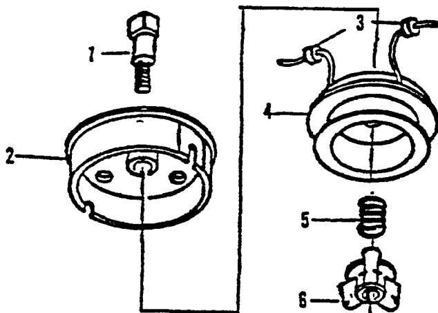
21560060 MANUAL HEAD
