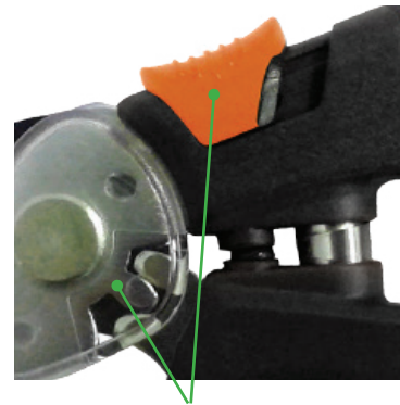
HP-43 Top Safety Lock and Gear Technology
