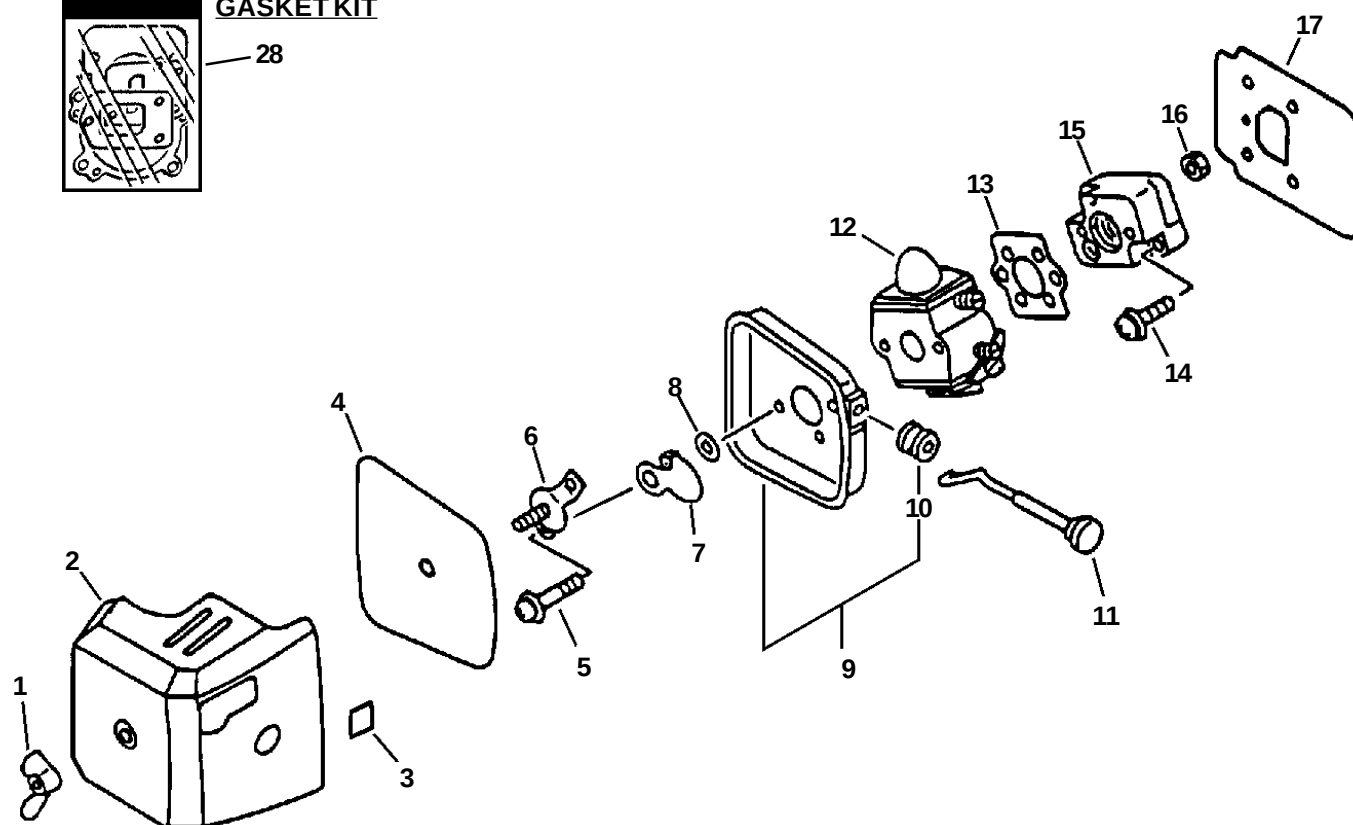
GASKET KIT
