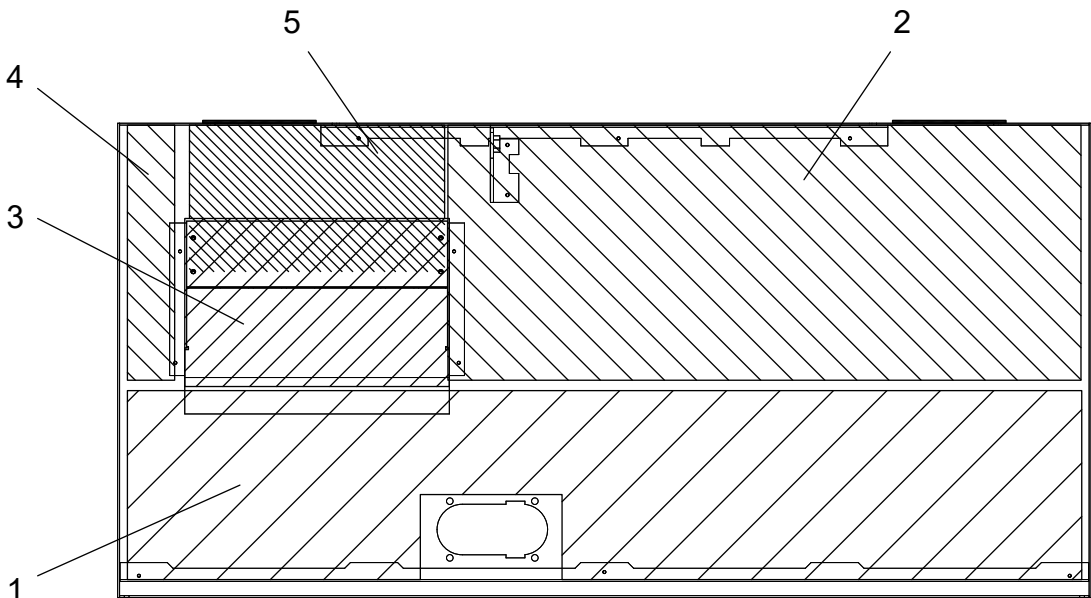
back view
