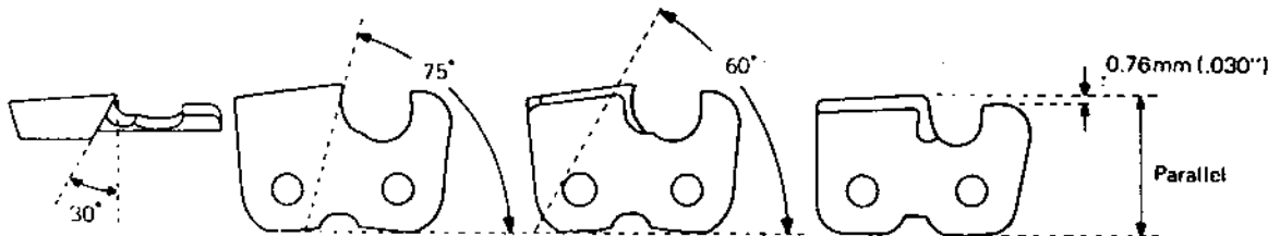
(Top plate cutting angle)
