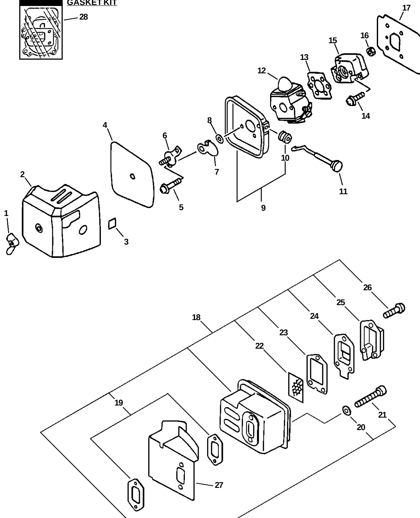
GASKET KIT
