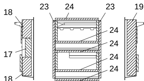
left view
