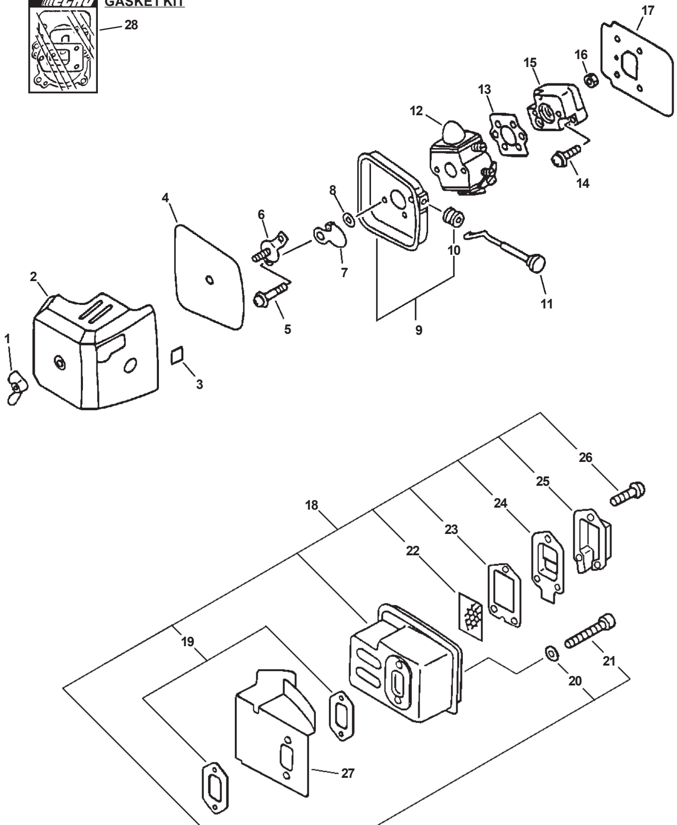
GASKET KIT
