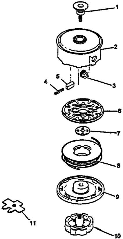
999442 00210 AUTOMATIC HEAD ASY
