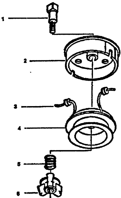
999442 00210 AUTOMATIC HEAD ASY
