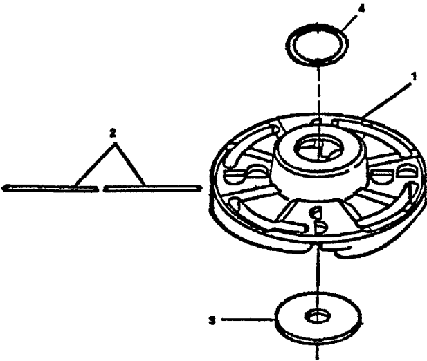
999442 00220 MANUAL HEAD ASY
